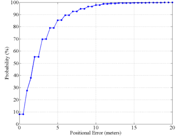
Figure 3. Position error cumulative probability distribution
