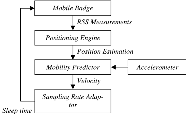
Figure 2. System architecture.
