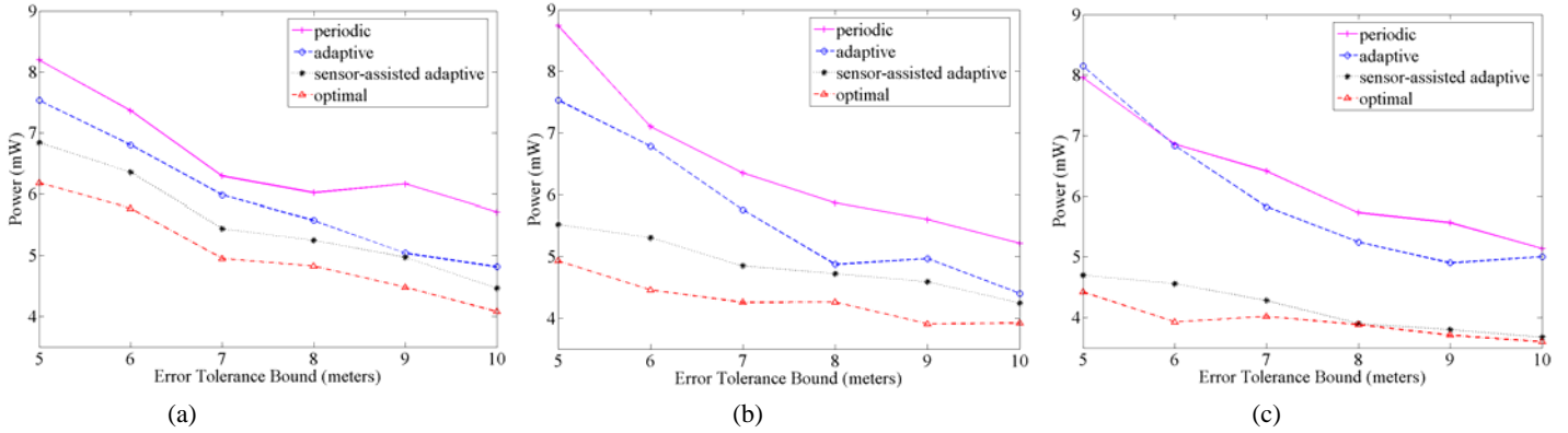
Figure 8. Tradeoff between power consumption and error tolerance under different mobility levels (70%, 50%, and 30%).
